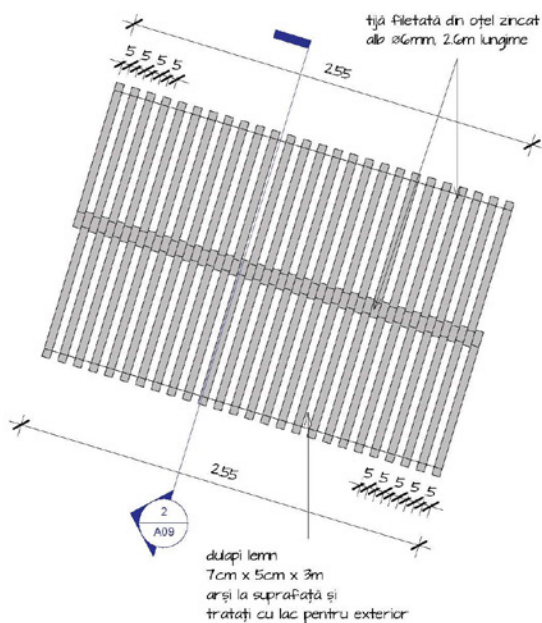
1 Plan "cabana" 1 : 25
